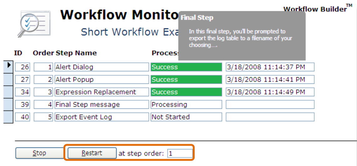
Figure 8: Restart Option
