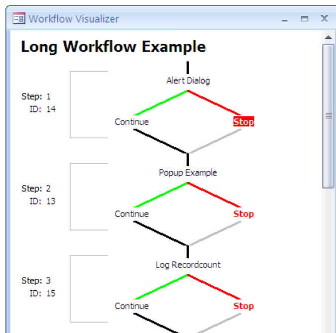
Figure 4: Workflow Visualizer
